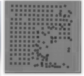
X-Ray Image of Migrated Die
